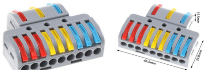
Cable range:0.08-4.0mm 2 /28-12AWG3in to 9out
