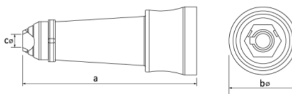
Öçüler / Dimensions (mm)
