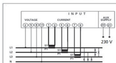
4-wire three-phase network
