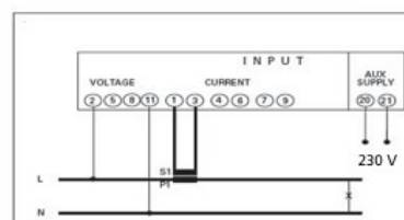
Single-phase network
