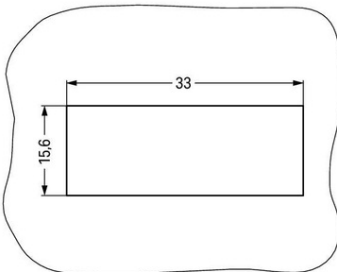
Plate thickness: 0.5 ... 2 mm Cutout tolerance: + 0.1 mm
