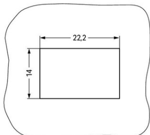
Plate thickness: 0.5 ... 2 mm Cutout tolerance: + 0.1 mm
