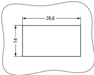
Plate thickness: 0.5 ... 2 mm Cutout tolerance: + 0.1 mm
