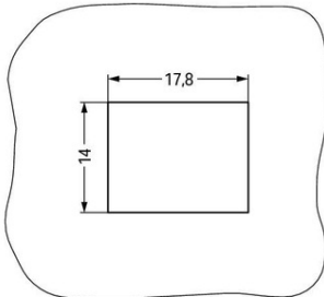
Plate thickness: 0.5 ... 2 mm Cutout tolerance: + 0.1 mm
